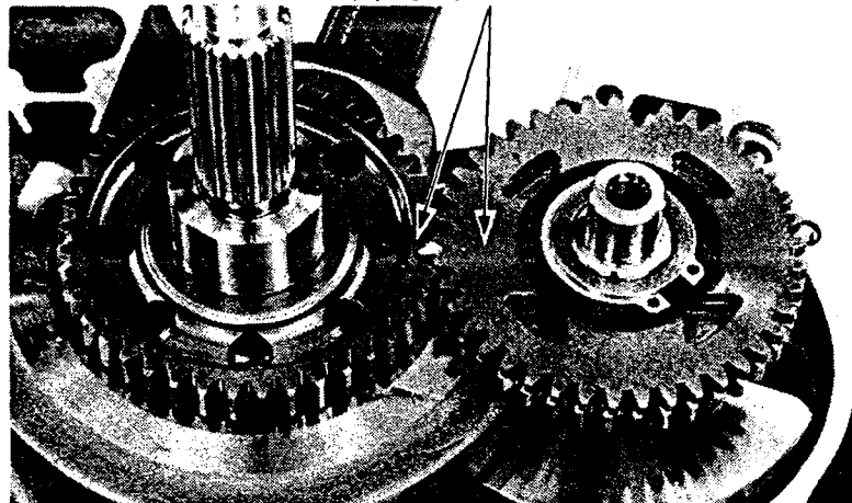
(1) PUNCH MARKS
