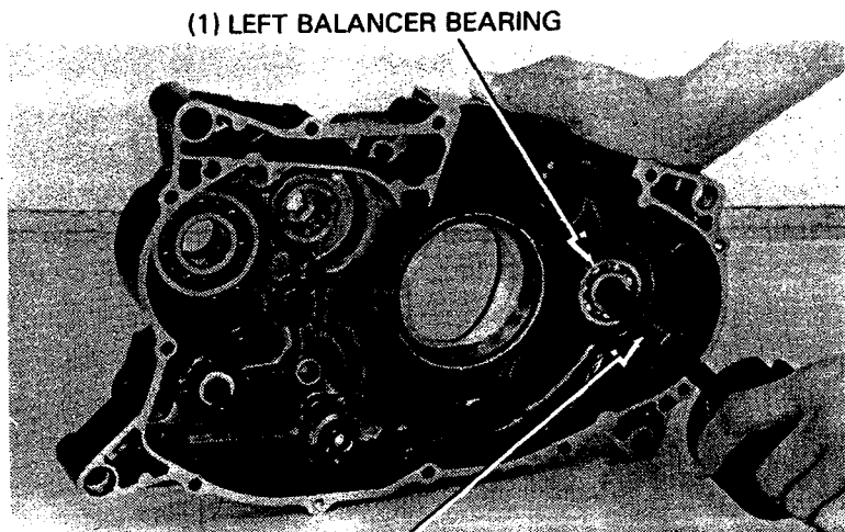
(2) BEARING REMOVER, 17 mm 07936-3710300
