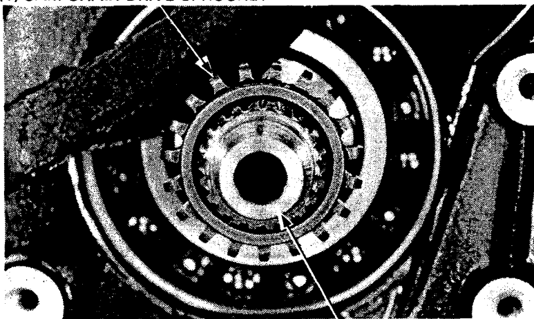
(2) CRANKSHAFT
