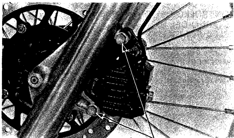
(1) MOUNTING BOLTS
